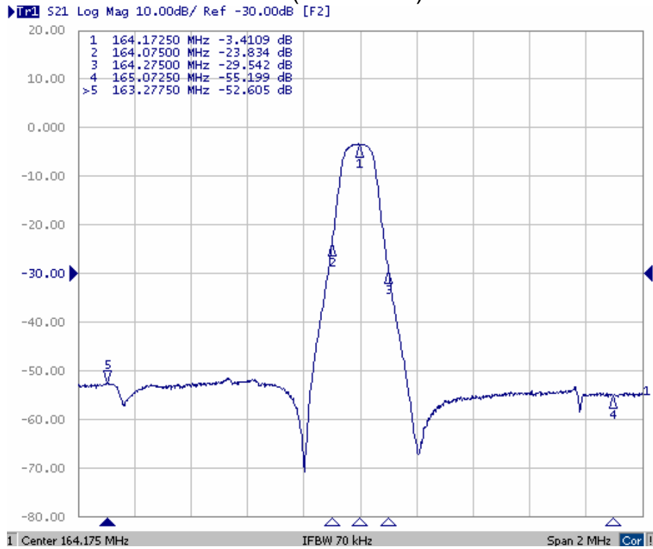
S21 (Inband)
