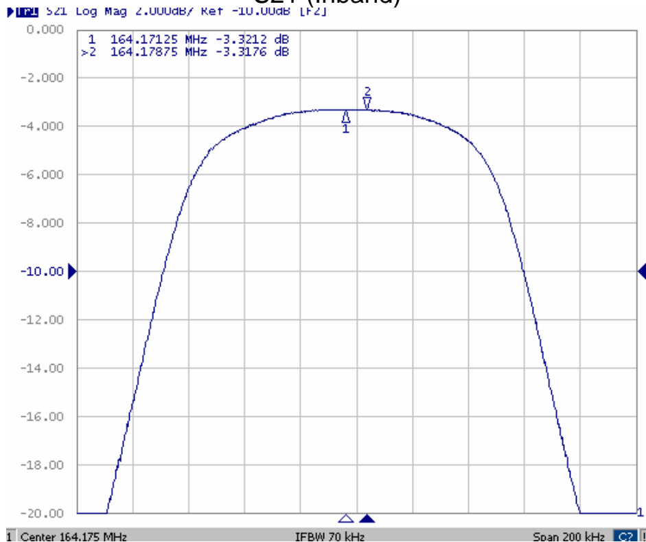
S21 (Inband)
