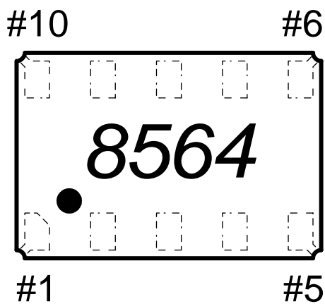
C3 Package: (top view)
