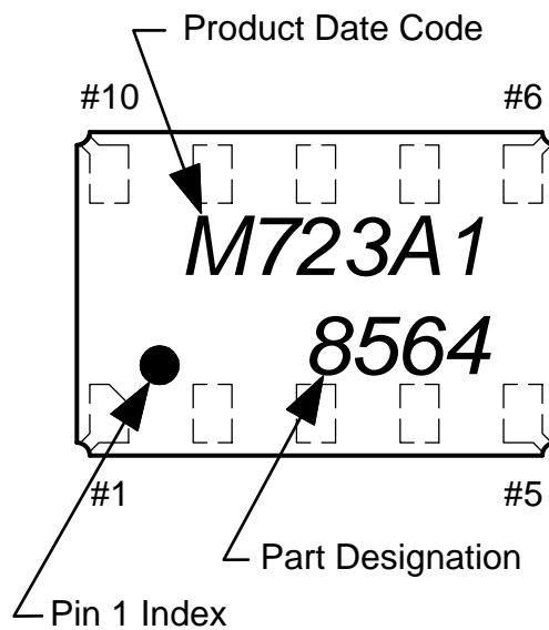
Laser marking RV-8564-C3 Package: (top view)
