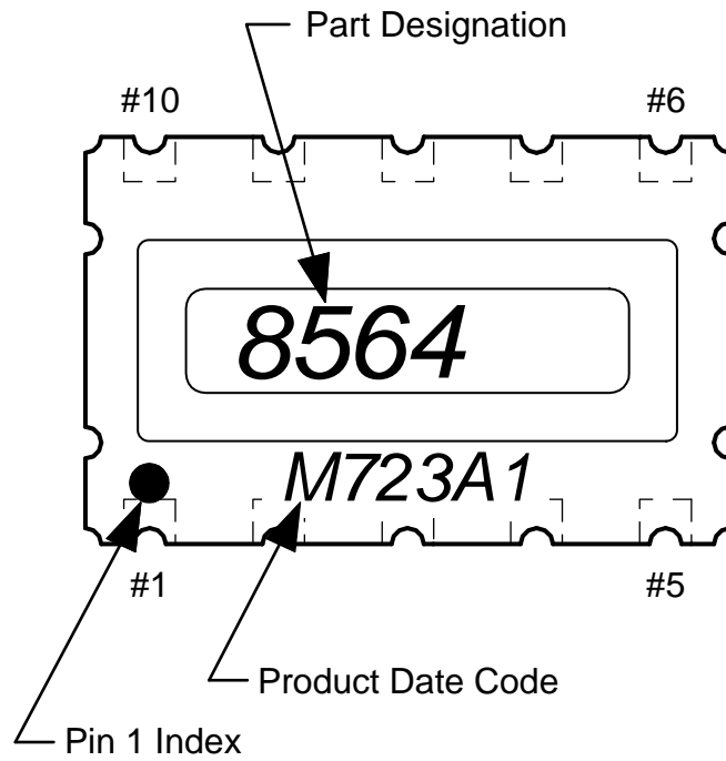
Laser marking RV-8564-C3 Package: (top view)
